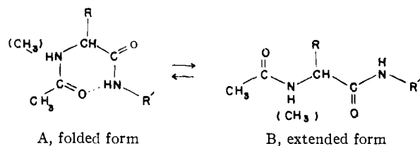
Fig. 1.—Two forms of the monomer of \text{CH}_3\text{CONHCHR-CONHR}' .
